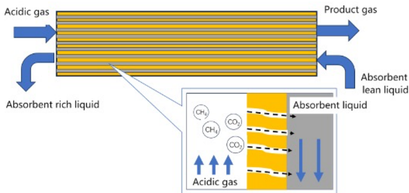
Figure 2. Schematic diagram of the absorption process of membrane contactors.
