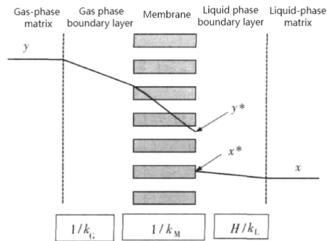
Figure 3. Schematic diagram of mass transfer in hollow fiber membrane contactor.
